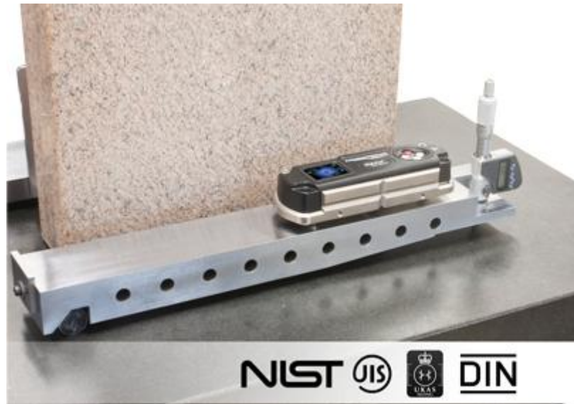
Digi-Pas ® Calibration equipment – Micrometer Sine Bar
